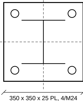
S-201 DETAIL 3: BP1
